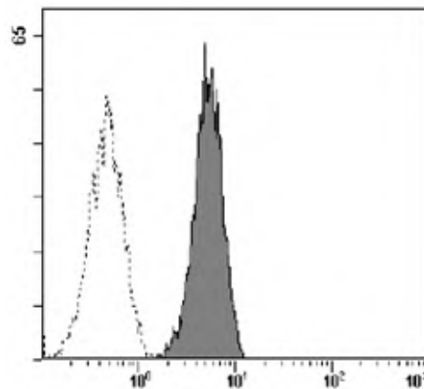
Flow cytometric analysis of human CRELD1 expression on Ba/F3 transfectant. Open histograms indicate the reaction of isotypic control to the cells. Shaded histograms indicate the reaction of W074-3 to the cells.
