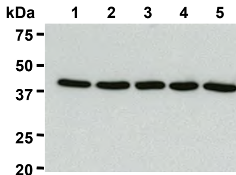
Western blot analysis of \beta -Actin in HeLa (1), NIH/3T3 (2), NRK (3), CHO (4) and MuH1 (5) using M177-3. Sample volume: 1 \mu g per lane
