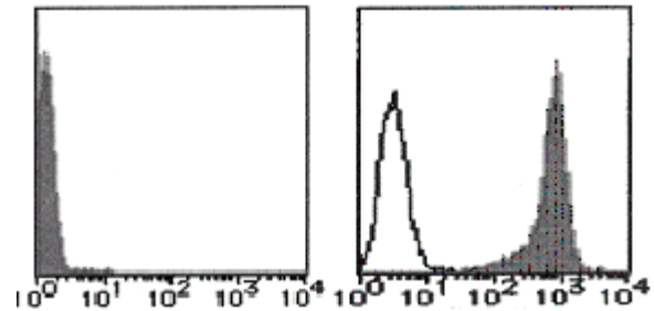
Flow cytometric analysis of HLA-A24 expression on LCL721 cells (right) and Jurkat cells (left). Open histogram indicate the reaction of isotypic control to the cells. Shaded histograms indicate the reaction of K0208-5 to the cells.
