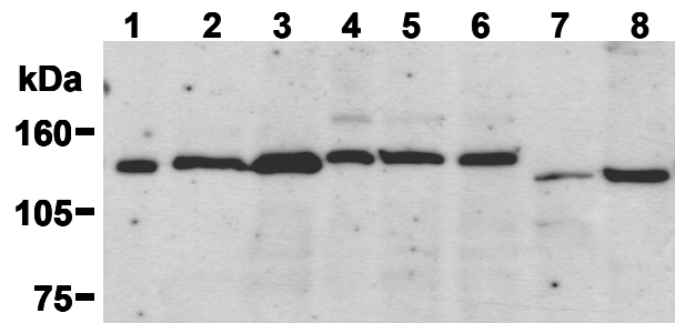
Western blot analysis of MORC3 expression in HL60 (1), U937 (2), A431 (3), WR19L (4), NIH/3T3 (5), MEF (6), Rat1 (7) and PC12 (8) using D238-3.
