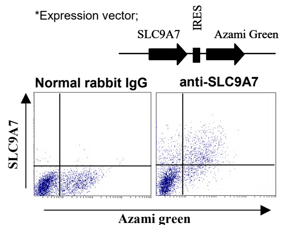
Flow cytometric analysis of intracellular SLC9A7 expression on 293T transiently expressing SLC9A7 and Azami green*. The staining intensity of BMP043 is shown in the vertical axis with Azami Green fluorescence on the horizontal axis.
